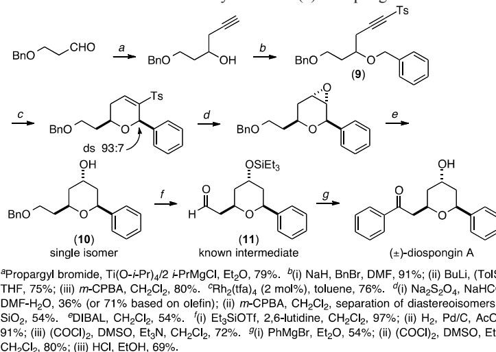
Scheme 3. Total Synthesis of (±)-Diospongins A.
