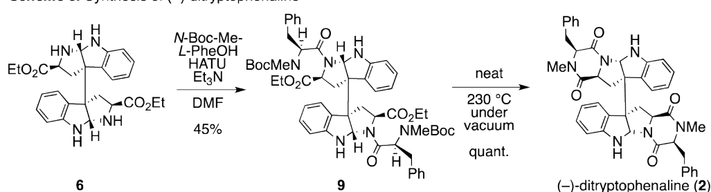
Scheme 3. Synthesis of (–)-ditryptophenaline
