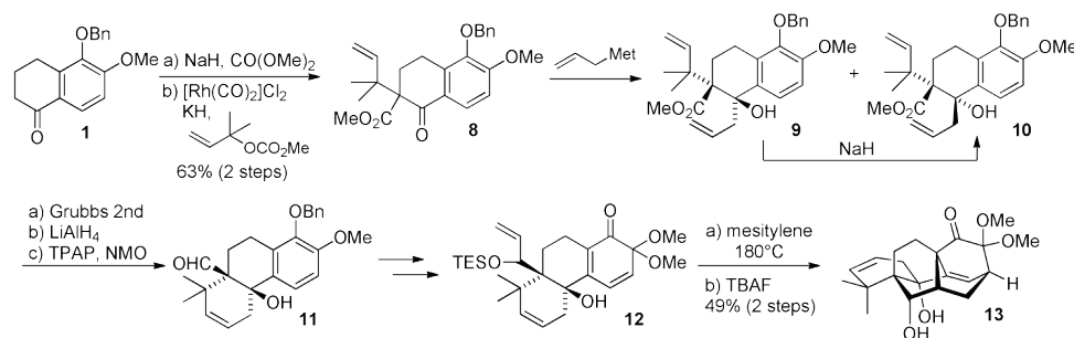
Figure 2. Construction of Pentacyclic Skeleton of Atropurpuran
