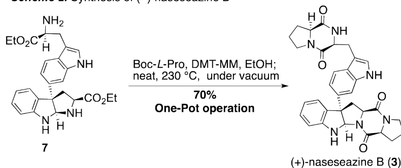
Scheme 2. Synthesis of (+)-naseaseazine B
