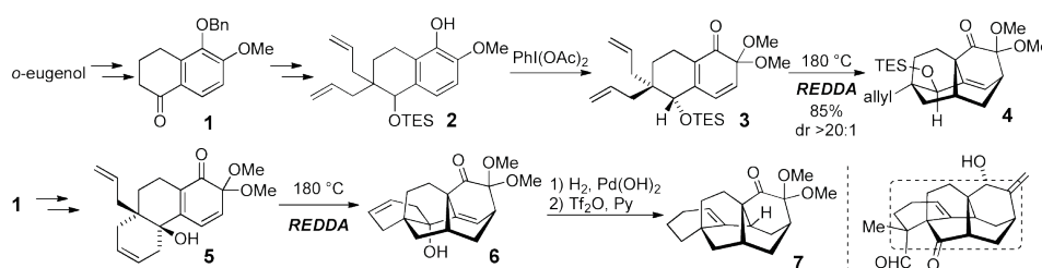
Figure 1. Construction of the Atropurpuran Skeleton using REDDA reaction
