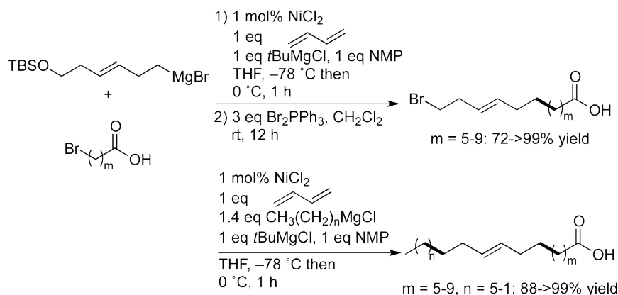
Scheme 1 Synthesis of elaidic acid and its regioisomers
