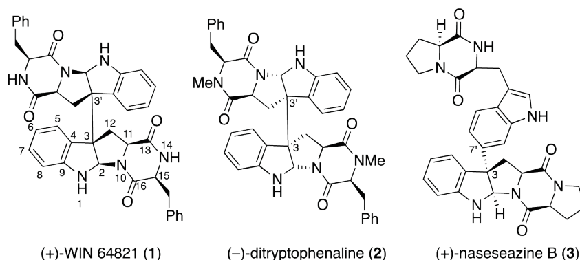
Figure 1. natural tryptophan-based dimeric diketopiperazine alkaloids
