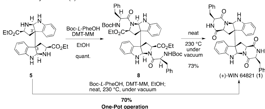
Scheme 1. Synthesis of (+)-WIN 64821
