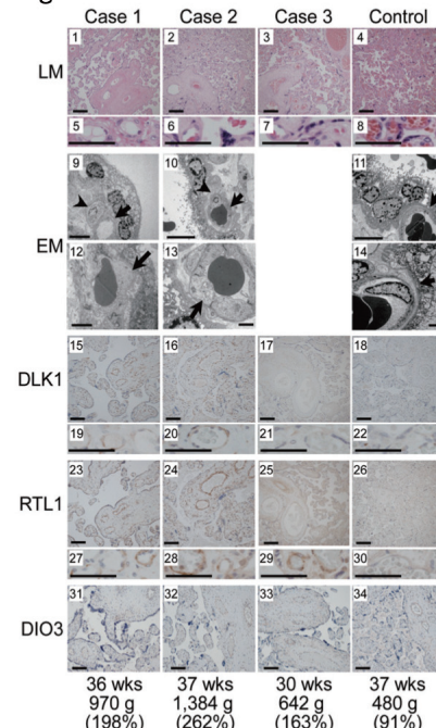
Fig 2. Histological examinations.
